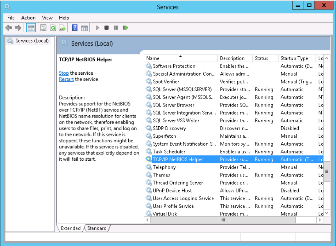
Figure 37 : Checking TCP/IP NetBIOS Helper service status (Windows Server)
