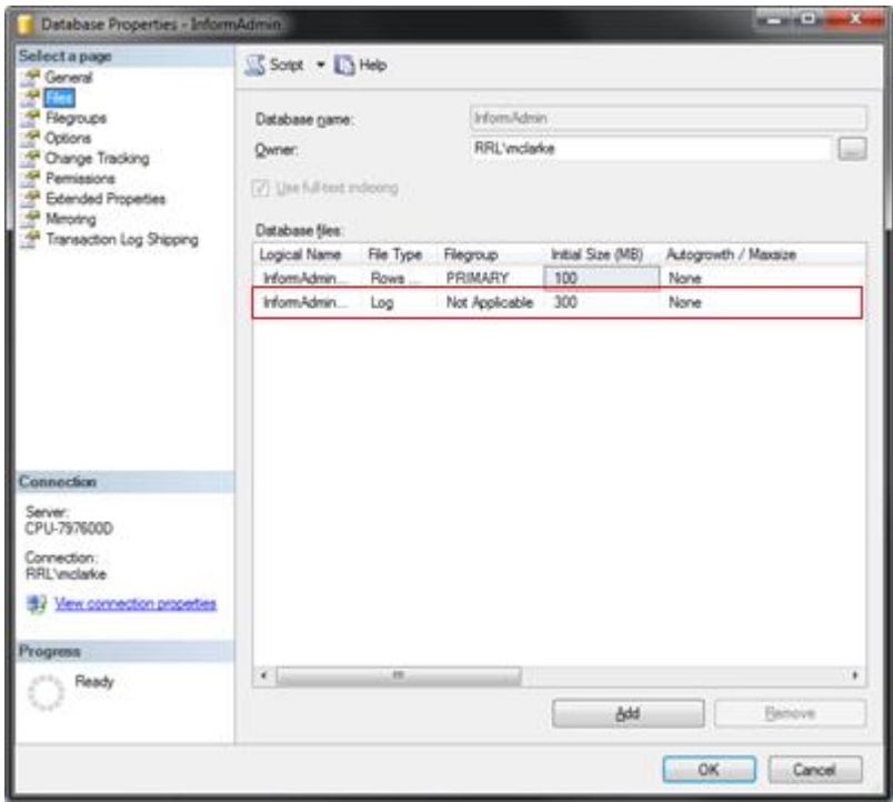
Figure 30 :SQL Management Studio – InformAdmin Properties dialog
