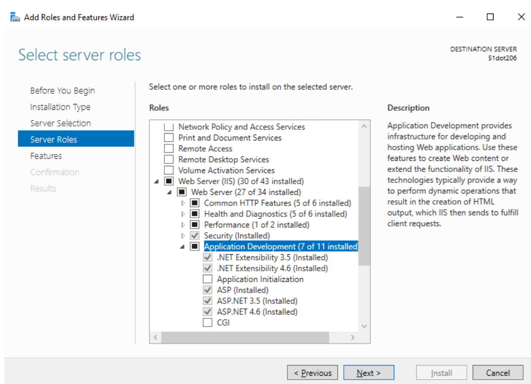
Figure 12: Add Roles and Features Wizard
