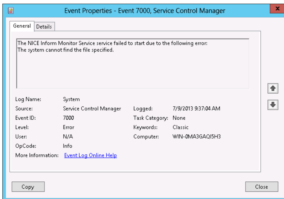
Figure 5: Event Properties
