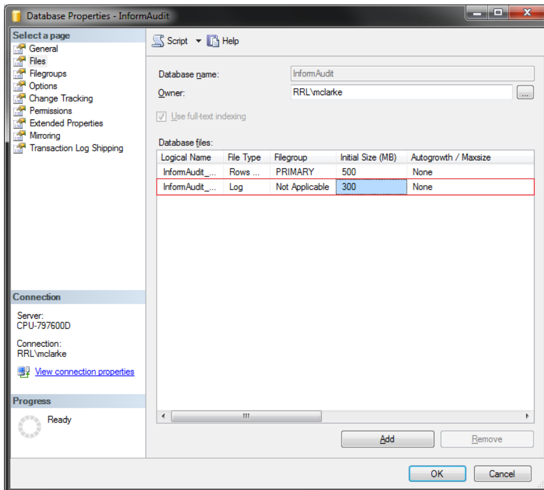
Figure 3232 : SQL Management Studio – opening InformAudit properties
