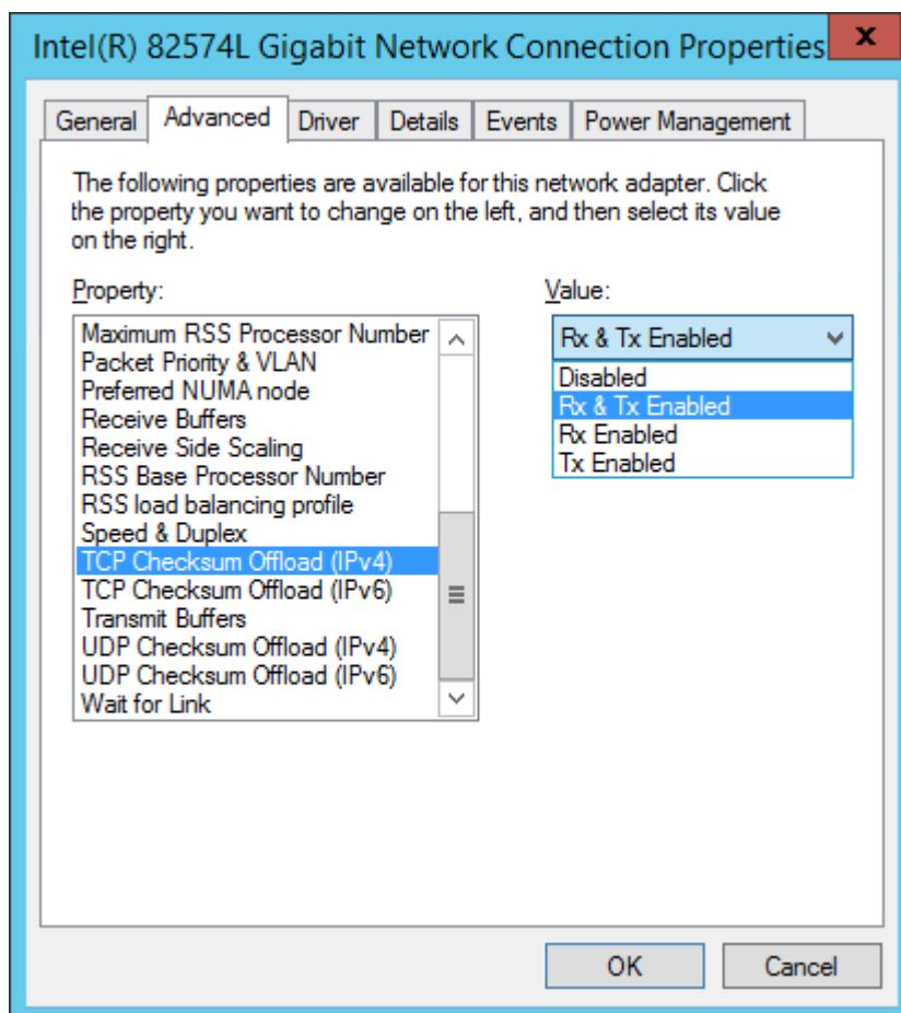
Figure 9: Configuring NIC checksum offload value
