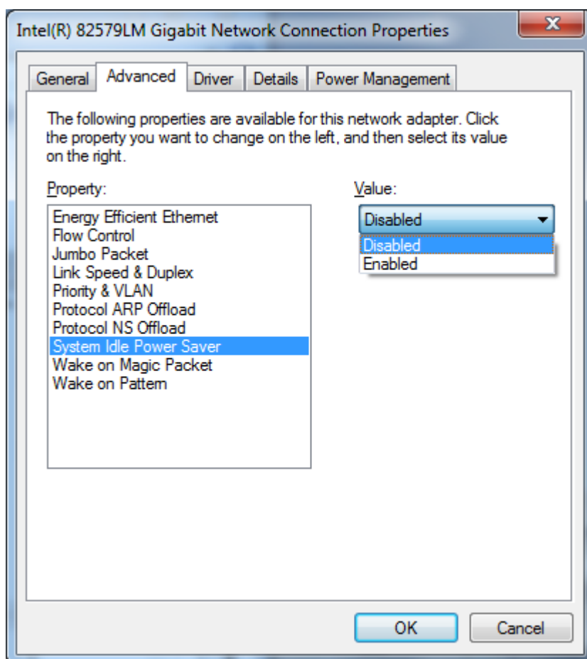
Figure 11: Configuring NIC system idle power saver value
