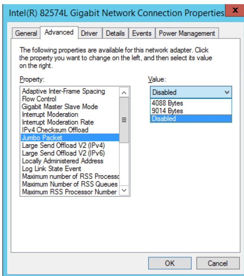
Figure 9: Configuring NIC jumbo packet value
