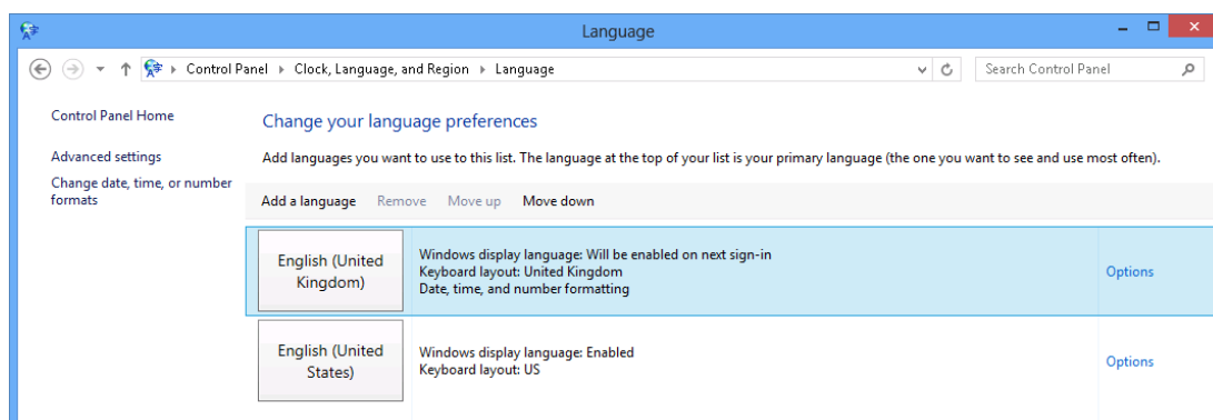
Figure 21: Language screen
